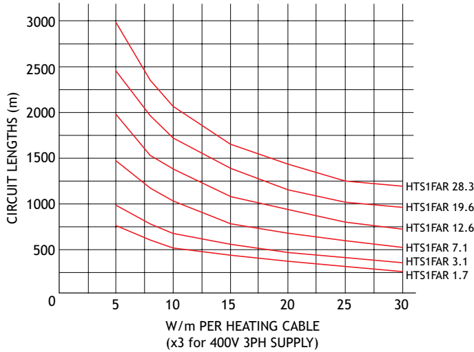
CIRCUIT LENGTH v POWER OUTPUT for 3PH SYSTEMS CONNECTED TO A 400V, 3PH SUPPLY
