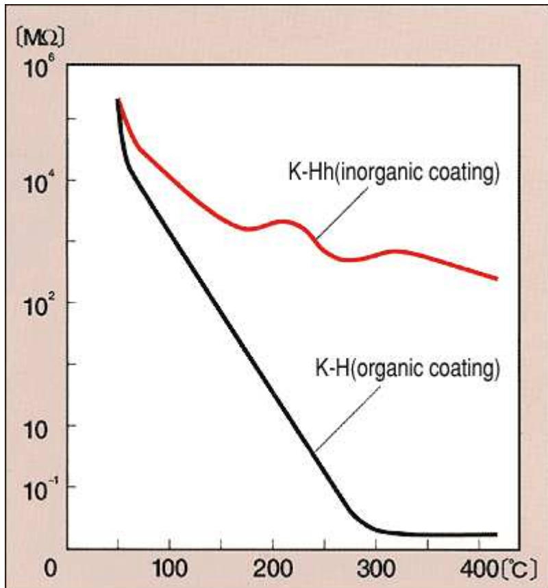
Graph 2: Temperature-Insulation Resistance
